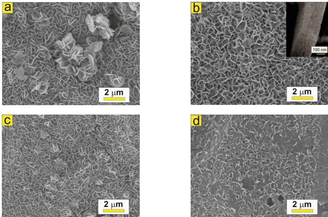
Fig.3. SEM images of simonkolleite precursors (a, c) deposited from water-ethanol solution containing \text{Zn}(\text{NO}_3)_2 and \text{KCl} with (a) and without PVP (c) and ZnO powders after annealing (b, d)
