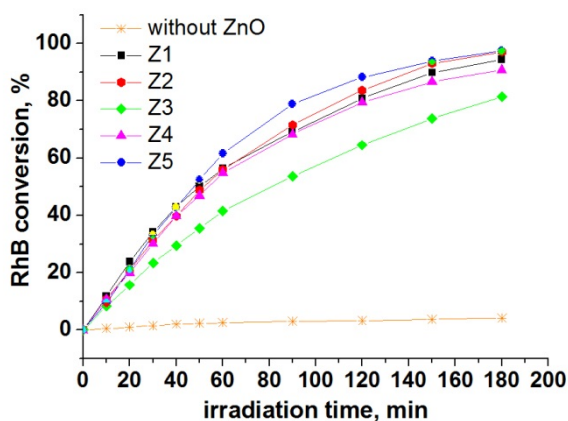
Fig. 6. Photodegradation of RhB over ZnO powders
