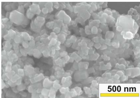
Fig. 4 SEM image of ZnO powder produced from aqueous solution containing \text{Zn}(\text{NO}_3)_2 , \text{KCl} and PVP.
