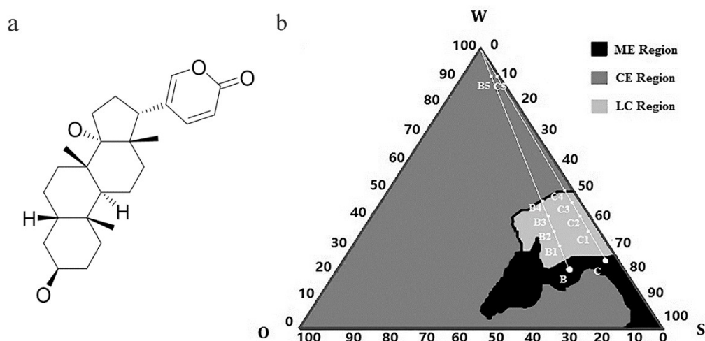
Fig. 1. (a) Chemical structure of the bufanolide steroid drug bufalin (BUF). (b) A pseudo-ternary phase diagram MCT/HS 15–Span 80/water [18] with an indication of the investigated O/S/W compositions along the dilution lines at 37 °C, which are chosen between the regions of microemulsions (ME), liquid crystals (LC), and coarse emulsions (CE). The phase transitions from ME to LC are examined by SAXS along the lines B–B5 and C–C5 upon progressive addition of water.
