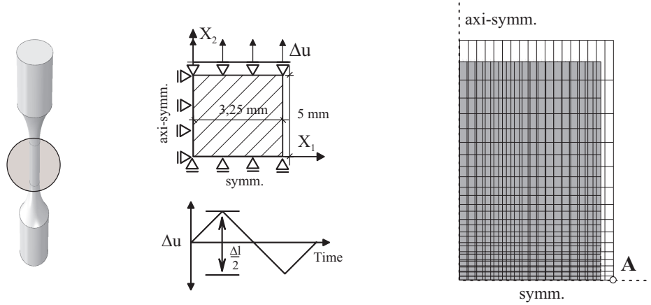
Figure 1: (a) Picture of the smooth round bar; (b) loading conditions; (c) finite element discretization.
