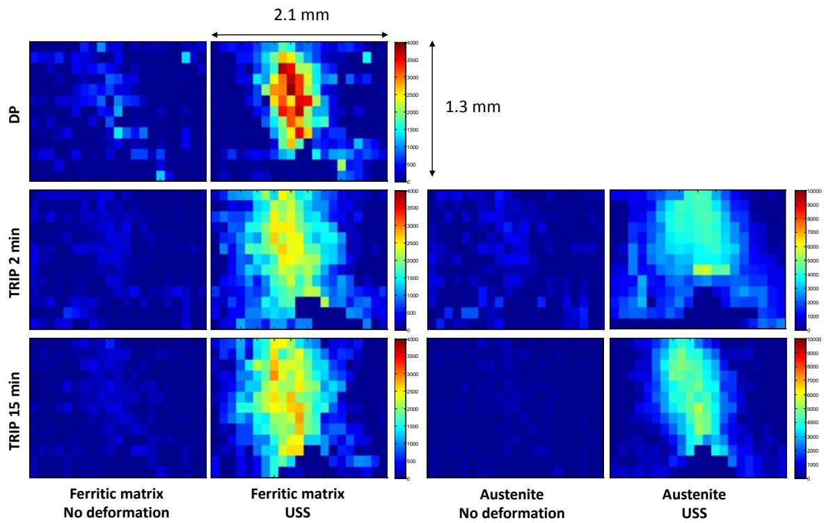
Figure 6 Spatial maps of the elastic shear strain \varepsilon_{12} ( 10^{-6} ) in the ferritic matrix and the austenite at no deformation and at USS for the DP, TRIP-2min and TRIP-15min samples.
