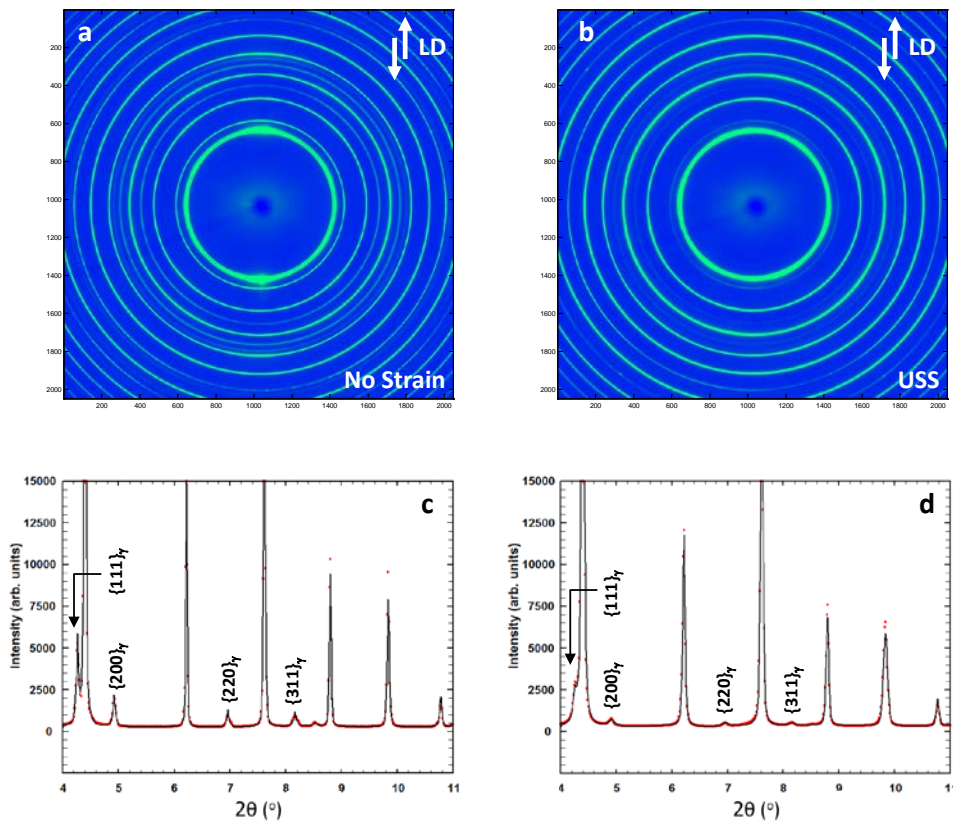
Figure 3 2D X-ray diffraction patterns at (a) no strain and (b) ultimate shear strength (USS). The loading direction (LD) is indicated in the figure. The 2D patterns have been subsequently integrated over the azimuth angles to obtain the one-dimensional X-ray patterns as a function of the scattering angle at (c) no strain and (d) ultimate shear strength. The corresponding Rietveld refinement of the one-dimensional X-ray patterns is also shown. The studied \{111\}_\gamma , \{200\}_\gamma , \{220\}_\gamma and \{311\}_\gamma austenite reflections have been labeled on the 1D patterns.
