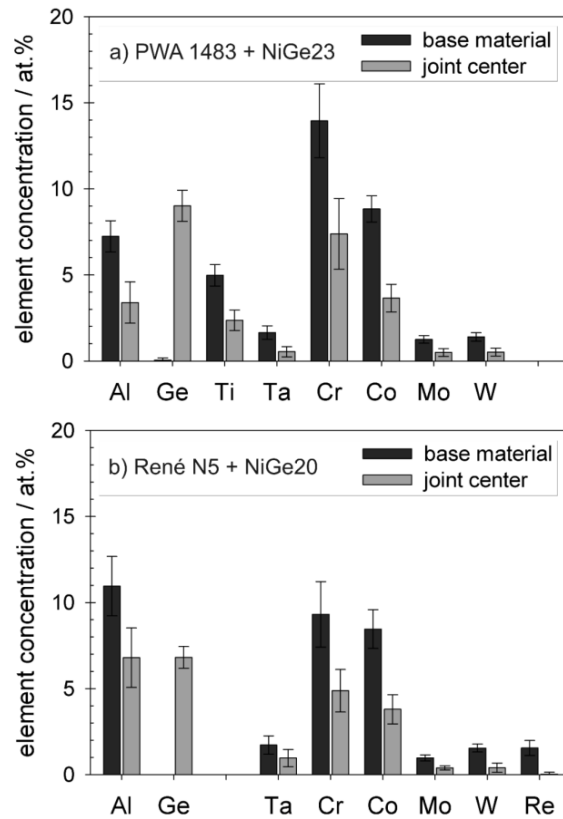
Figure 6: Results of the EDX analysis of the two brazing of a) PWA 1483 + NiGe23 and b) René N5 + NiGe20. Plotted are base material and the joint center for both systems.
