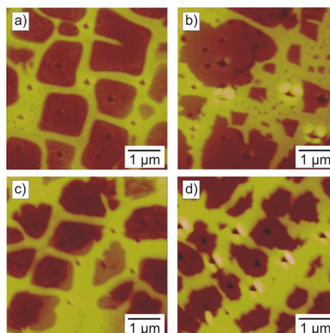
Figure 2: AFM-images of the microstructures after the brazing heat treatment including nanoindentations in the \gamma and \gamma' phase: a) center of the brazing zone of PWA 1483 with NiGe23, b)
