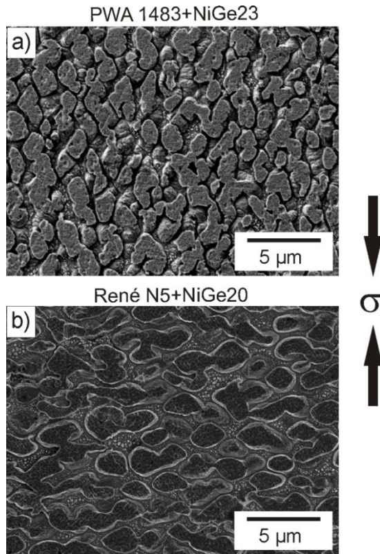
Figure 7: Microstructure in the joint region after creep under compression at 1000 °C with applied loads of a) 150 MPa for PWA 1483 + NiGe23 and b) 200 MPa for René N5 + NiGe20.
