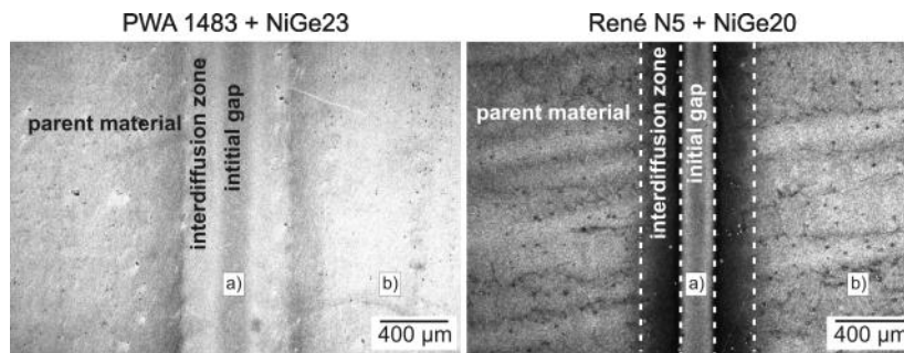
Figure 1: Light micrograph (dark field images) of the brazing zone of PWA 1483 with NiGe23 and René N5 with NiGe20. The positions where the hardness measurements were performed in the joint area and base material are indicated by letters a and b, respectively.
