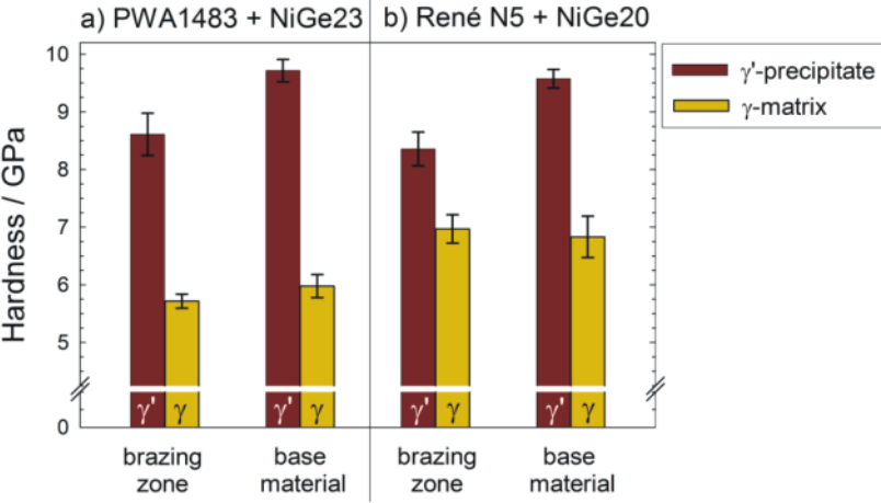
Figure 3: Nanoindentation results for the brazings of a) PWA 1483 + NiGe23 and b) René N5 + NiGe20.
