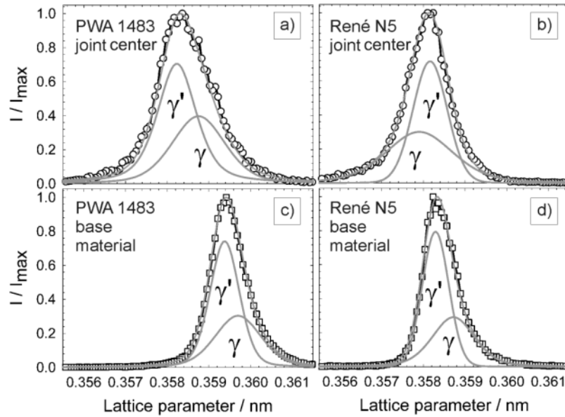
Figure 5 XRD-Profiles for the measurements within the joint region a) and b) and the base material c) and d) for PWA 1483 + NiGe23 a) and c) and René N5 + NiGe20 b) and d).
