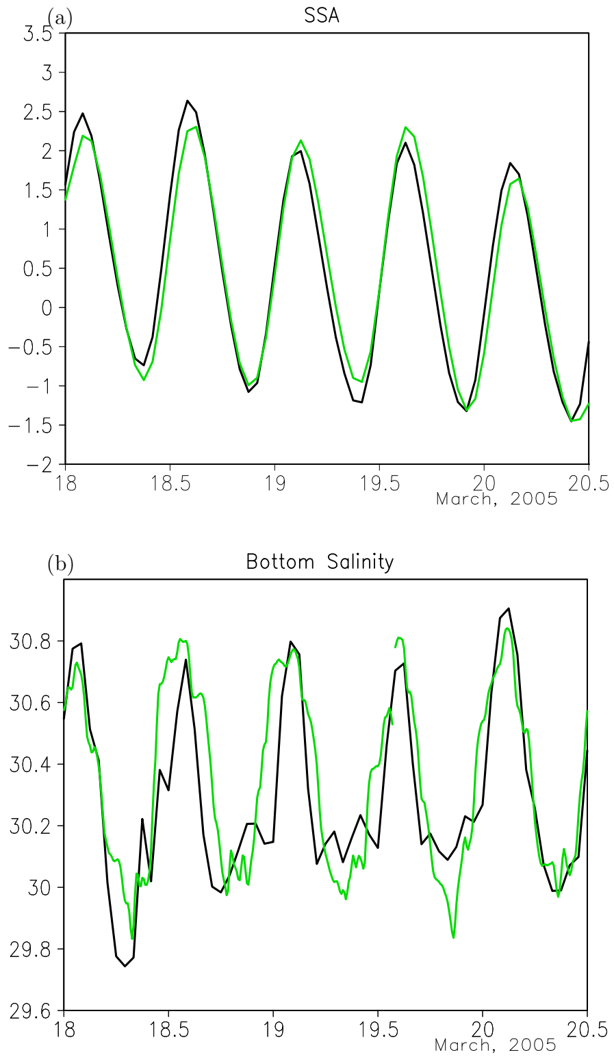
Fig. 13. Comparison at the WATT data station: green line-WATT station observations, black line-simulations plotted at the location of the station. (a) Sea surface anomaly (meters), (b) bottom salinity (psu).
