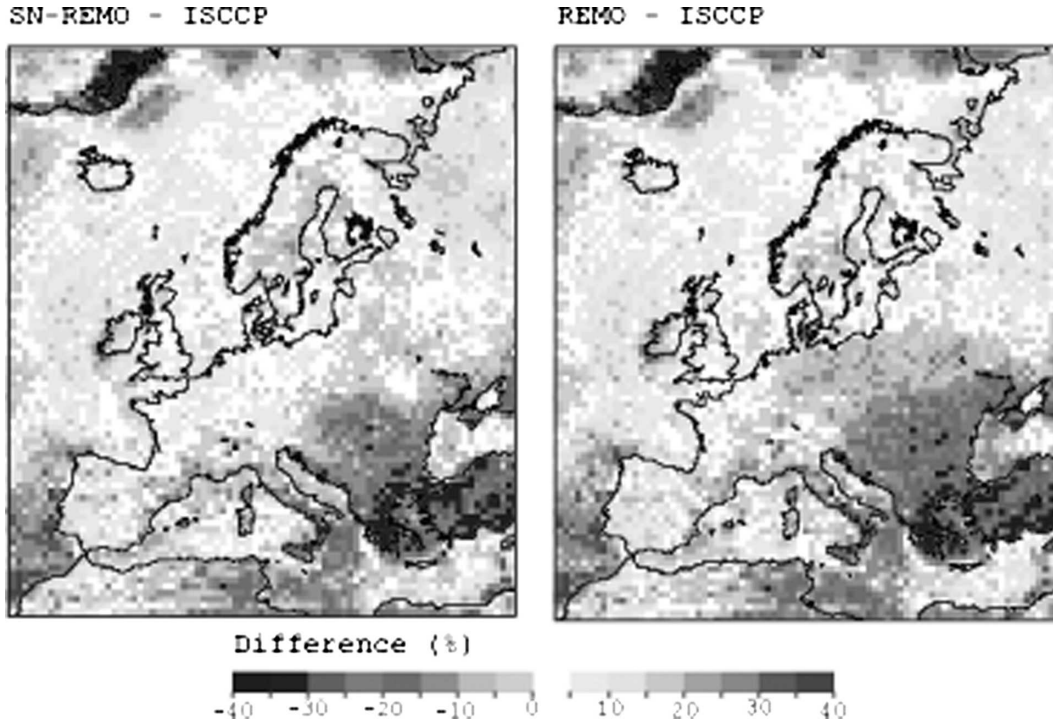
FIG. 4. Mean difference between simulated and satellite-derived cloud amount. (left) SN-REMO minus ISCCP and (right) REMO minus ISCCP.
