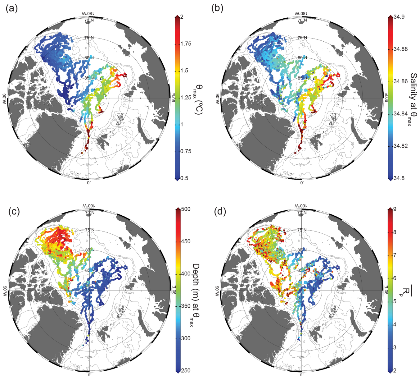
Figure 5. (a) Map of \theta_{max} ( ^{\circ}\text{C} ) across the Arctic Basin. (b) Map of salinity at \theta_{max} . (c) Map of depth (m) at \theta_{max} . (d) Map of \overline{R_p} . As Atlantic Water circulates around the basin, its core \theta_{max} and salinity at core \theta_{max} decrease, while its depth at core \theta_{max} and \overline{R_p} increase.
