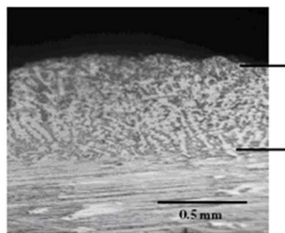
Fig. 17 Cross section micrograph of CO 2 laser nitrated titanium (from [103]).
