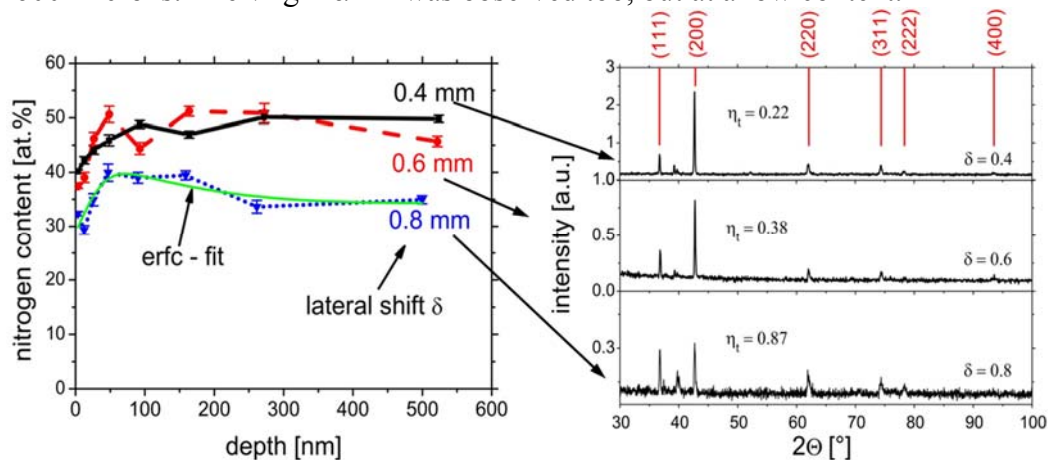
Fig. 11 Nitrogen depth profiles using different lateral shifts \delta (left) and their corresponding diffraction pattern (right) (from [60]). \eta_t describes the intensity ration of the (111) to the (200) peak and is known as the texture parameter.
