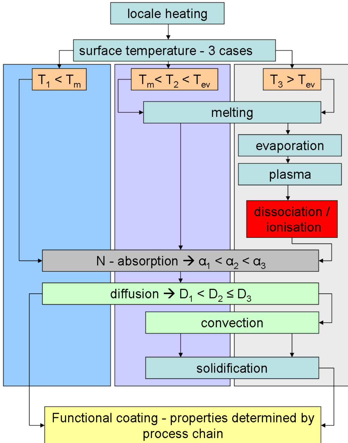
Fig. 2 Determination of different process chains depending on the surface temperature T_i - ( T_m - melting point, T_{ev} - evaporation point, \alpha_i -absorption coeff., D_i - diffusion coeff.).
