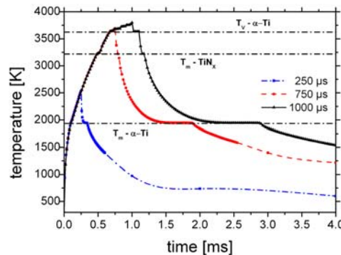
Fig. 14 Surface temperature development during a macropulse [59].
