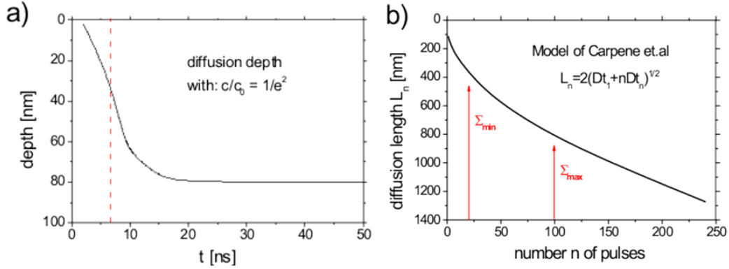
Fig. 9 Diffusion depth (drop of the concentration to 1/e^2 ) for the irradiation with Nd:YAG laser pulse a) as well as the diffusion length L for the irradiation with n pulses b) according to the model of [49]. D and t correspond to the respective diffusion coefficient and times. \Sigma corresponds the overlapping in the experiments.
