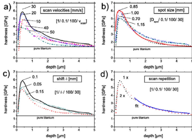
Fig. 5 Influence of a) the scan velocity v_{scan} , b) the spot size D_{spot} , c) the lateral shift \delta , and d) the scan repetition n on the measured hardness. In d), an example of a Jönsson and Hogmark [116] fit is shown (fit). For all plots, the parameters are given by the notation [D_{spot} [\text{mm}] / \delta [\text{mm}] / f [\text{Hz}] / v_{scan} [\text{mm/s}] (from [57]).
