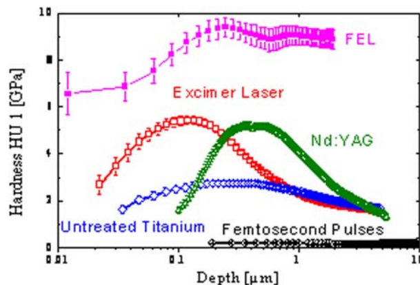
Fig. 19 Hardness of Ti:Sapphire laser nitrided titanium in comparison to other laser treatments.
