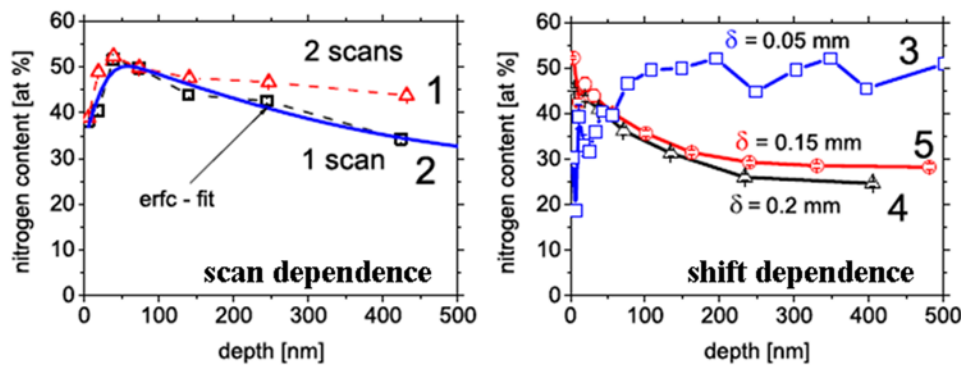
Fig. 6: Nitrogen depth profiles for two scans n (left) as well as for different lateral shifts (right) with the following parameters ( n , D_b = 1 mm, \delta = 0.05 - 0.2 mm, v = 30 mm/s and f = 100 Hz), from [57]
