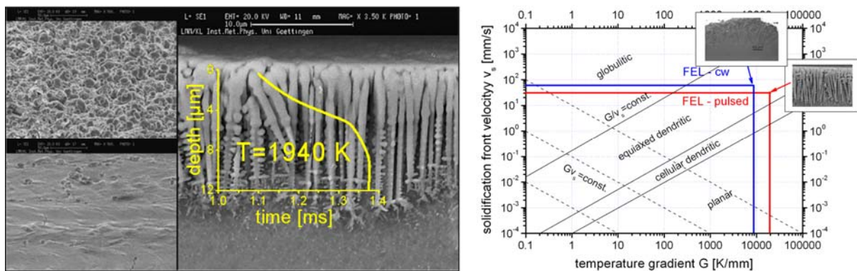
Fig. 20 Solidification behaviour, melting temperature isotherm (TiN) of pulsed FEL nitrided titanium [left] and classification of the solidification behaviour [right] of FEL laser nitrated titanium into the theory in [124].
