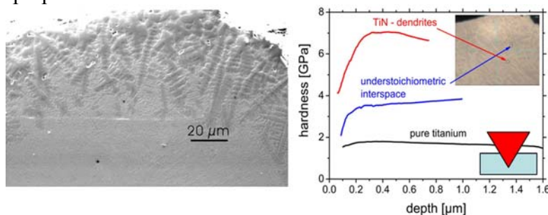
Fig. 12 Cross section micrographs of titanium nitride and hardness measurements at different regions (from [60]).
