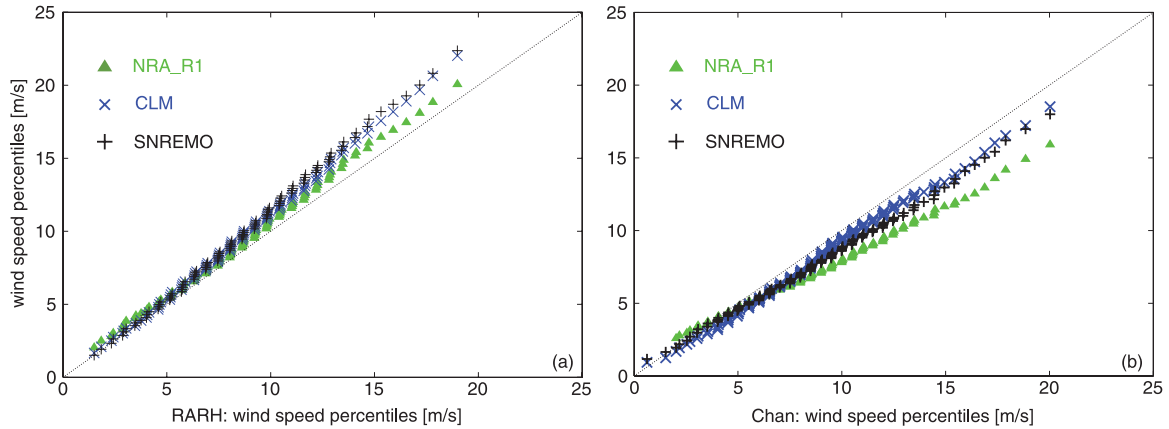
FIG. 5. Percentile–percentage distributions of wind speed in 1998, measured ( x axis) vs NRA_R1, SN-REMO and CLM percentiles at (a) the buoy RARH as an open-ocean station and (b) the light ship English Channel as a coastal station. The 99 symbols (triangles, crosses, and Xs for NRA_R1, SN-REMO, and CLM, respectively) represent the wind speed percentiles in steps of 1%. Thus, the first (last) symbol represents the 1st (99th) percentile and the wind speed below which 1% (99%) of all in situ and modeled wind speeds can be found, respectively. In the ideal case of perfect agreement between in situ and modeled wind speed frequency distributions, all percentiles would lie on the bisector line.
