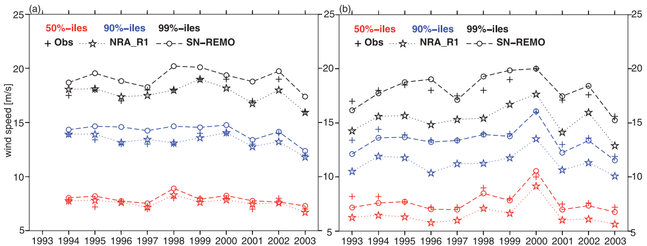
FIG. 6. Yearly percentiles of wind speed for (a) the platform F3 as an open-ocean station and (b) the light ship DeBu as a coastal station: observation (cross), NRA_R1 (dotted, star), and SN-REMO (dashed, circle). Red: 50%, blue: 90%, and black: 99%.
