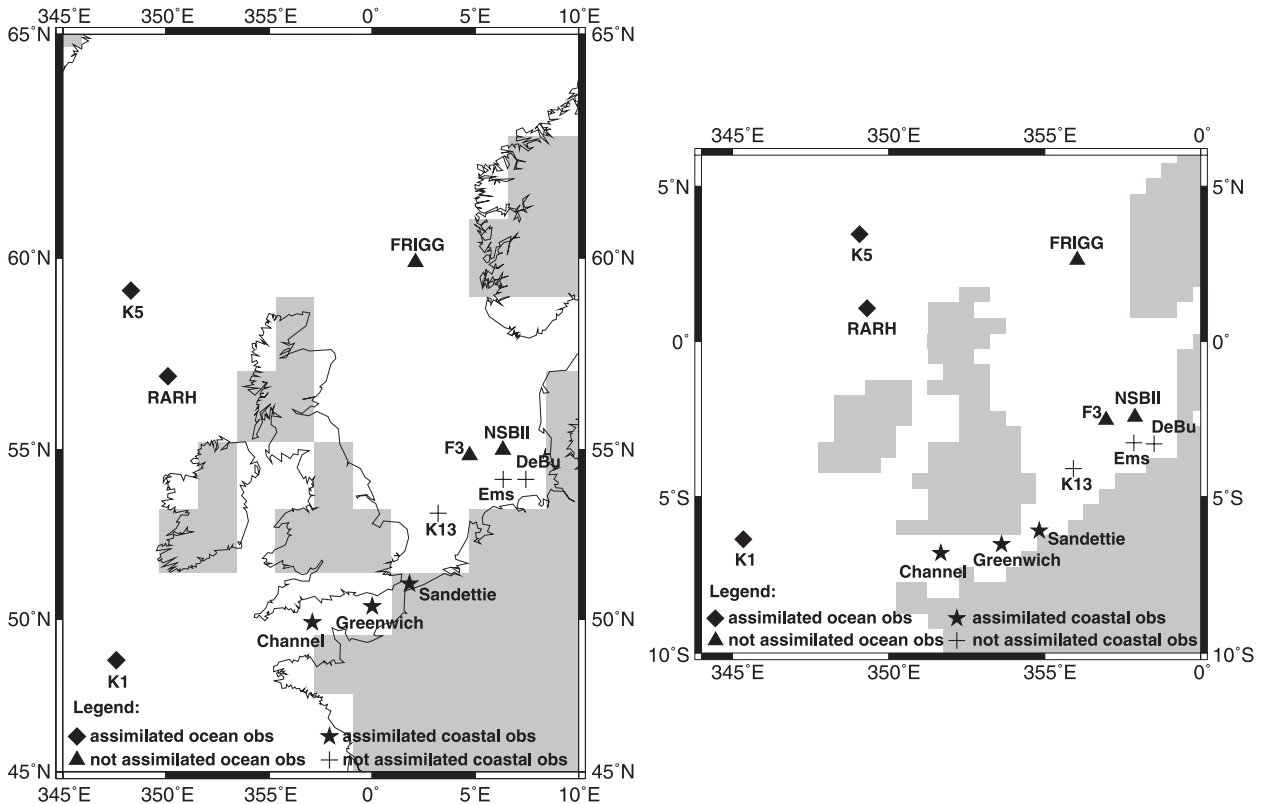
FIG. 2. Locations of wind speed observations (obs) over land-sea masks of (left) NRA_R1 and (right) REMO (rotated coordinate system).
