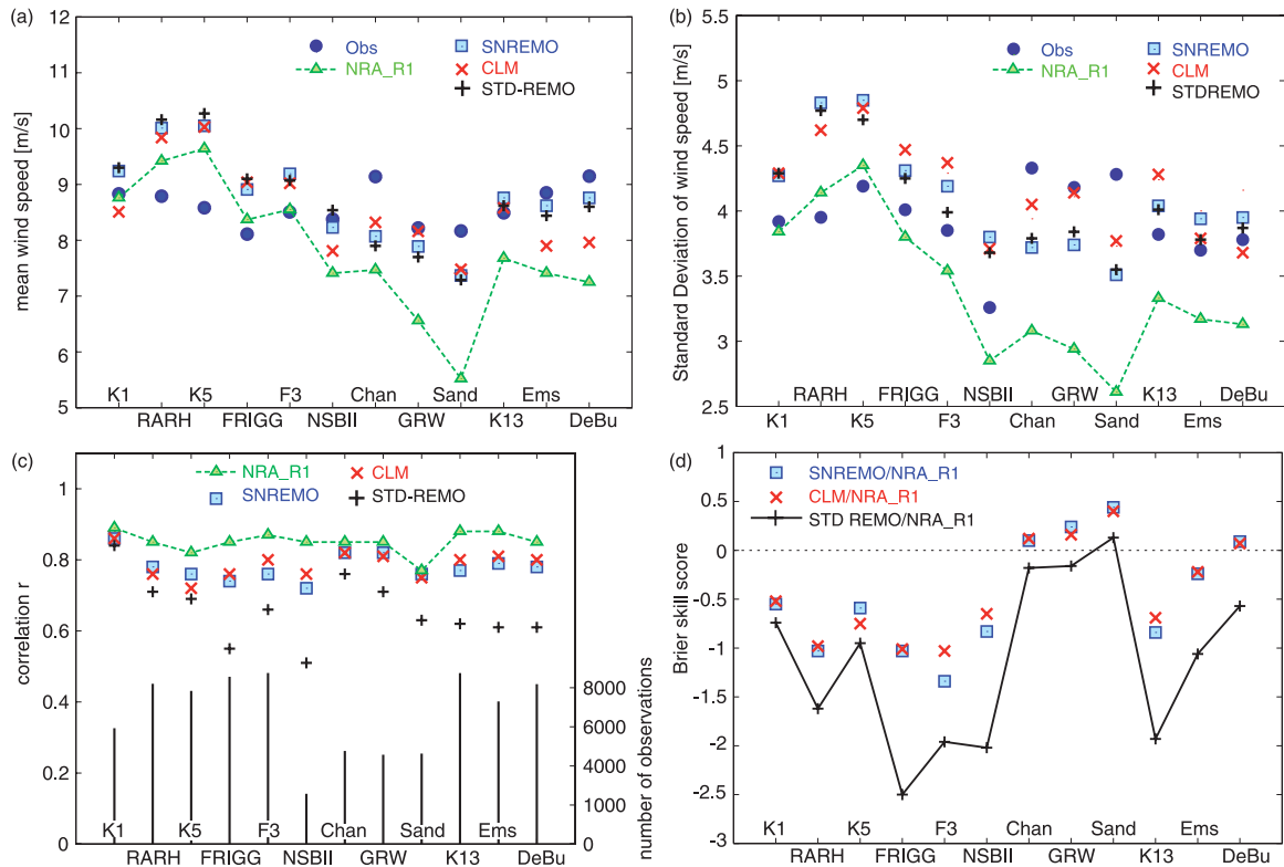
FIG. 3. Comparison of in situ, reanalyzed, and RCM-hindcast wind speed for 1998: (a) mean wind speed, (b) its std dev, (c) number of observations and correlation coefficient r , and (d) BSSs using NRA_R1 time series as reference forecast and SN-REMO, STD-REMO, and CLM time series as forecast.
